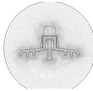
(ب): 62672 elements
