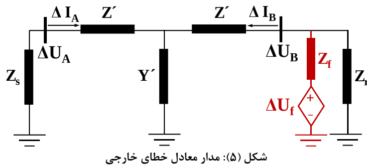
Figure (5): External fault equivalent circuit
